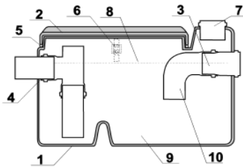
Schematic diagram of the grease trap SG series "Optima"
